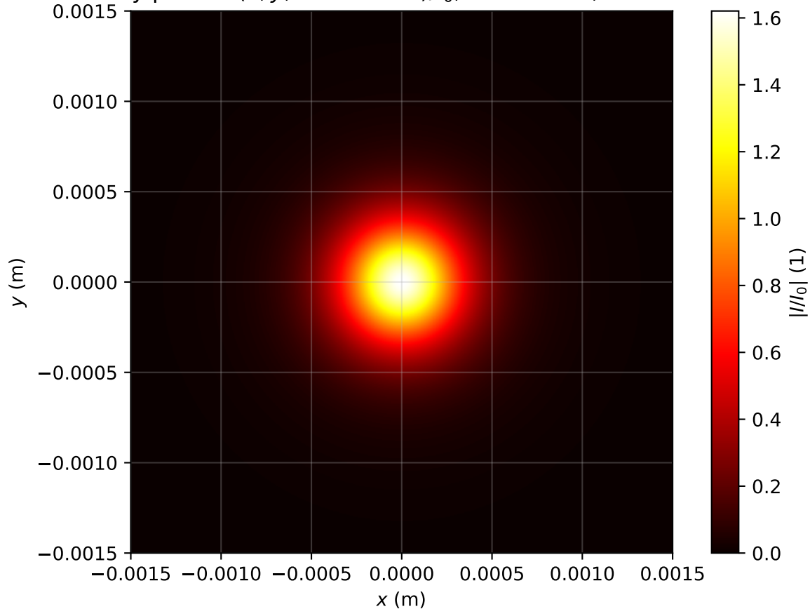
Intensity profile I(x, y, z = 1.831m)/I_0 , Pin=0.9Pcr, artificial time
